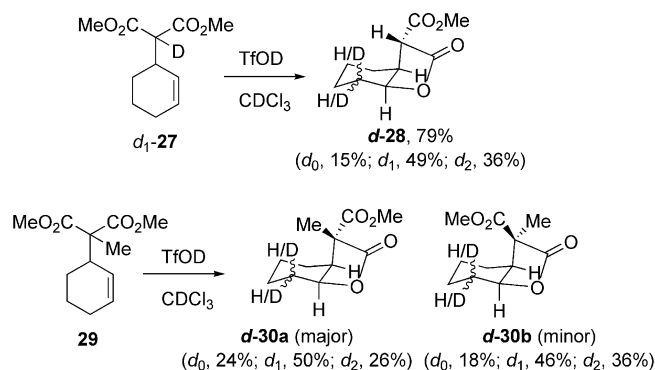
Scheme 13. Lactonisation of cyclohexylmalonates with TfOD. [23]
