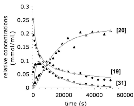
Figure 3. Graph of the reaction of 19 with TfOH. Experimental values: \blacklozenge = diallylmalonate ( 19 ); \blacksquare = intermediate ( 31 ); \blacktriangle = lactone ( 20 ). Calculated values: grey lines, see Scheme 11 for details.
