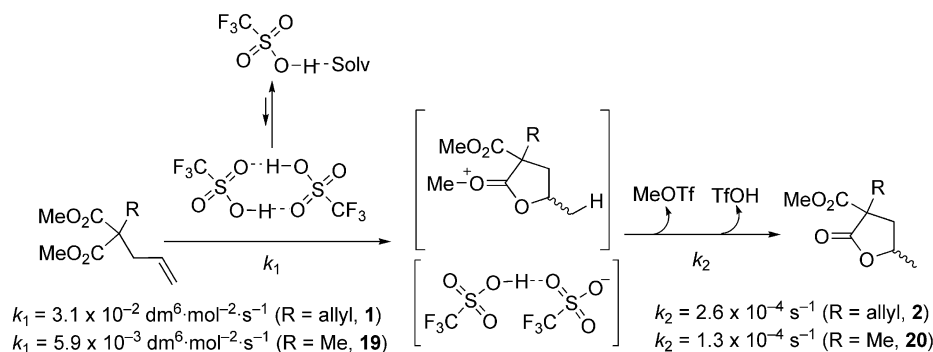
Scheme 11. Simplified two-step mechanism for the kinetics of lactonisation of di- and monoallylmalonates.
