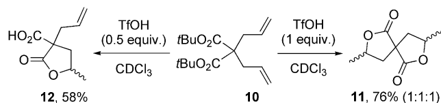
Scheme 6. Lactonisation of tert -butyl diallylmalonate ( 10 ).
