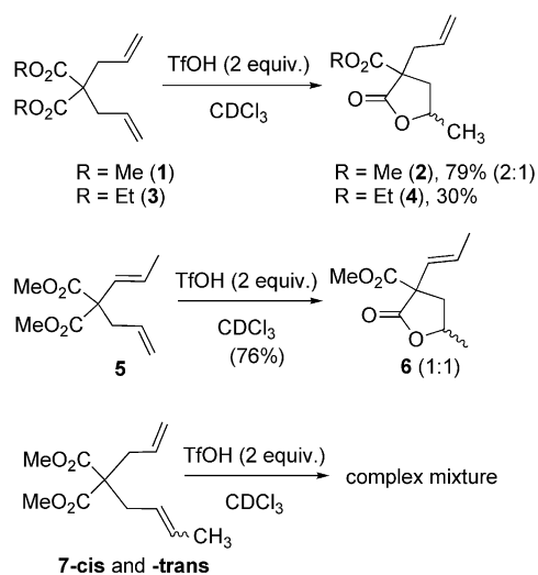
Scheme 4. Dealkylative monolactonisation of diallylmalonates.
