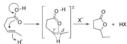
Scheme 1. Mechanism proposed for the lactonisation of olefinic acids. [3]
