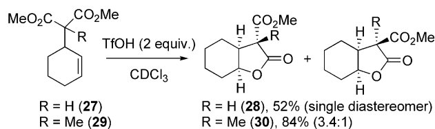
Scheme 10. Reaction of cyclic derivatives 27 and 29 with TfOH.
