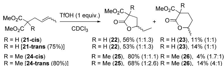
Scheme 9. Reaction of crotyl derivatives 21 and 24 with TfOH.
