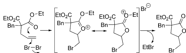
Scheme 3. Bromolactonisation of diethyl allyl(benzyl)malonate. [7]
