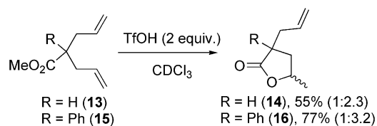
Scheme 7. Lactonisation with monoester derivatives 13 and 15 .
