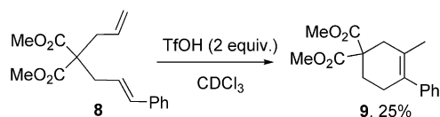
Scheme 5. Reaction of allyl(cinnamyl)malonate 8 with TfOH.
