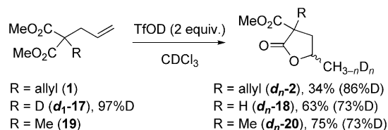
Scheme 12. Deuteration experiments with TfOD.
