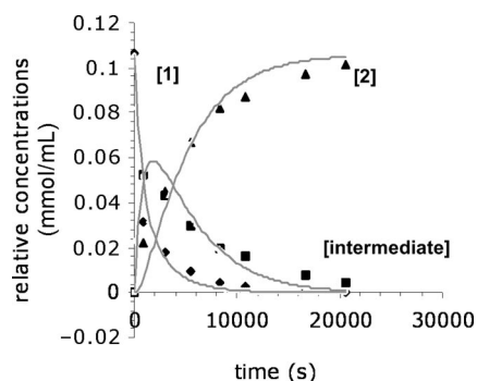
Figure 2. Graph of the reaction of 1 with TfOH. Experimental values: \blacklozenge = diallylmalonate ( 1 ); \blacksquare = intermediate; \blacktriangle = lactone ( 2 ). Calculated values: grey lines, see Scheme 11 for details.
