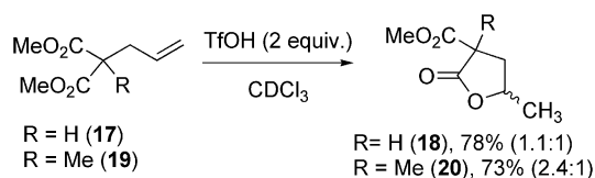
Scheme 8. Reaction of monoallylmalonates 17 and 19 with TfOH.
