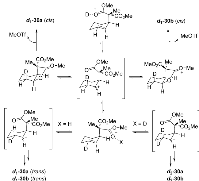
Scheme 14. Proposed isomerisation of oxonium intermediates to explain deuteration experiments. Lactone 30 is used as model.
