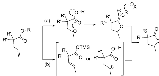
Scheme 2. Mechanisms proposed for the lactonisation of olefinic esters. [4,5]
