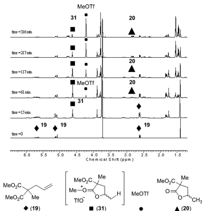
Figure 1. ^1\text{H} NMR spectra of the reaction of 19 with TfOH in \text{CDCl}_3 .
